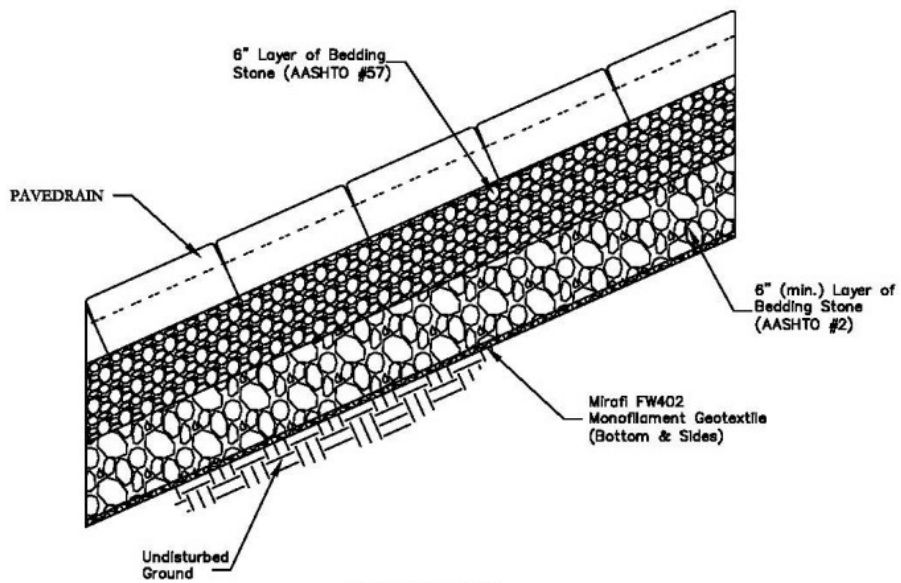
SLOPE-SECTION SIDE VIEW
