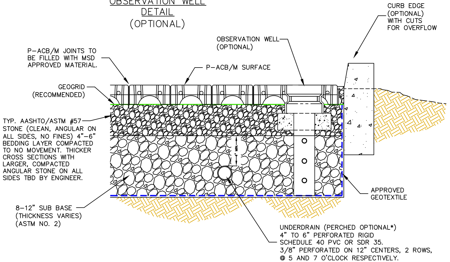
PERMEABLE - ARTICULATING CONCRETE BLOCK/MAT TYPICAL SECTION
