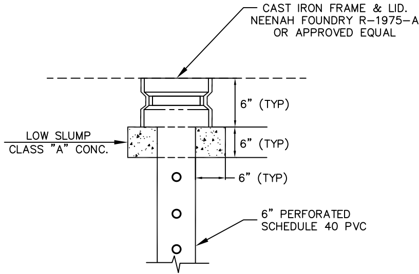
OBSERVATION WELL DETAIL (OPTIONAL)
