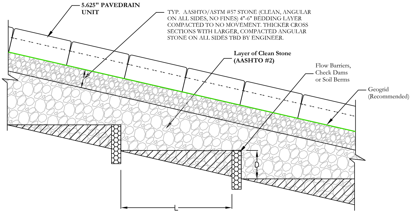
STEPPED INSTALLATION CROSS-SECTION N.T.S.
