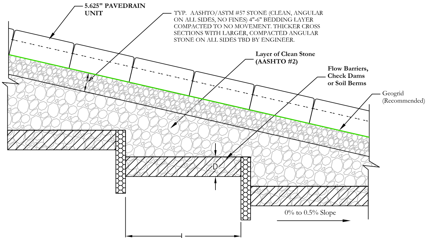
SLOPED INSTALLATION CROSS-SECTION N.T.S.
