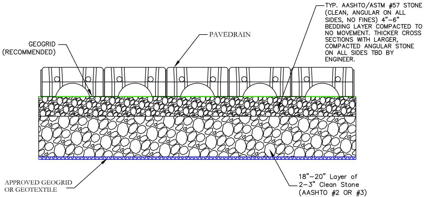
CROSS-SECTION END VIEW
