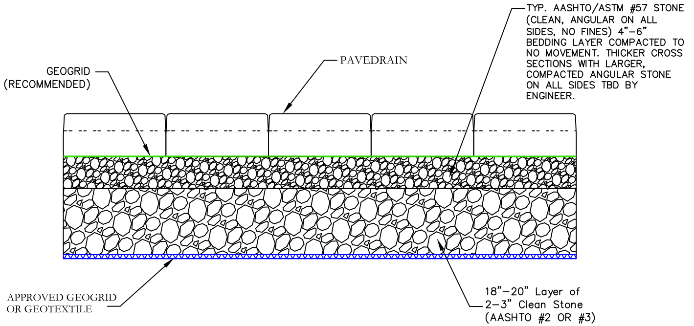
CROSS-SECTION SIDE VIEW
